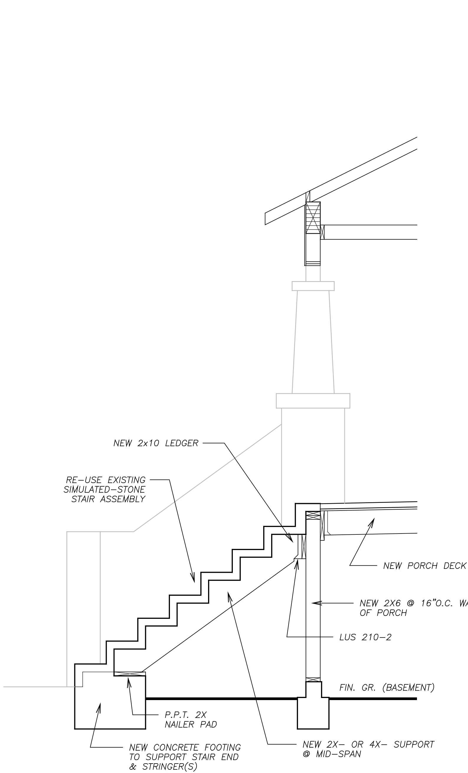
1 SEC. @ STAIRS SCALE: 1/2" = 1'-0"
