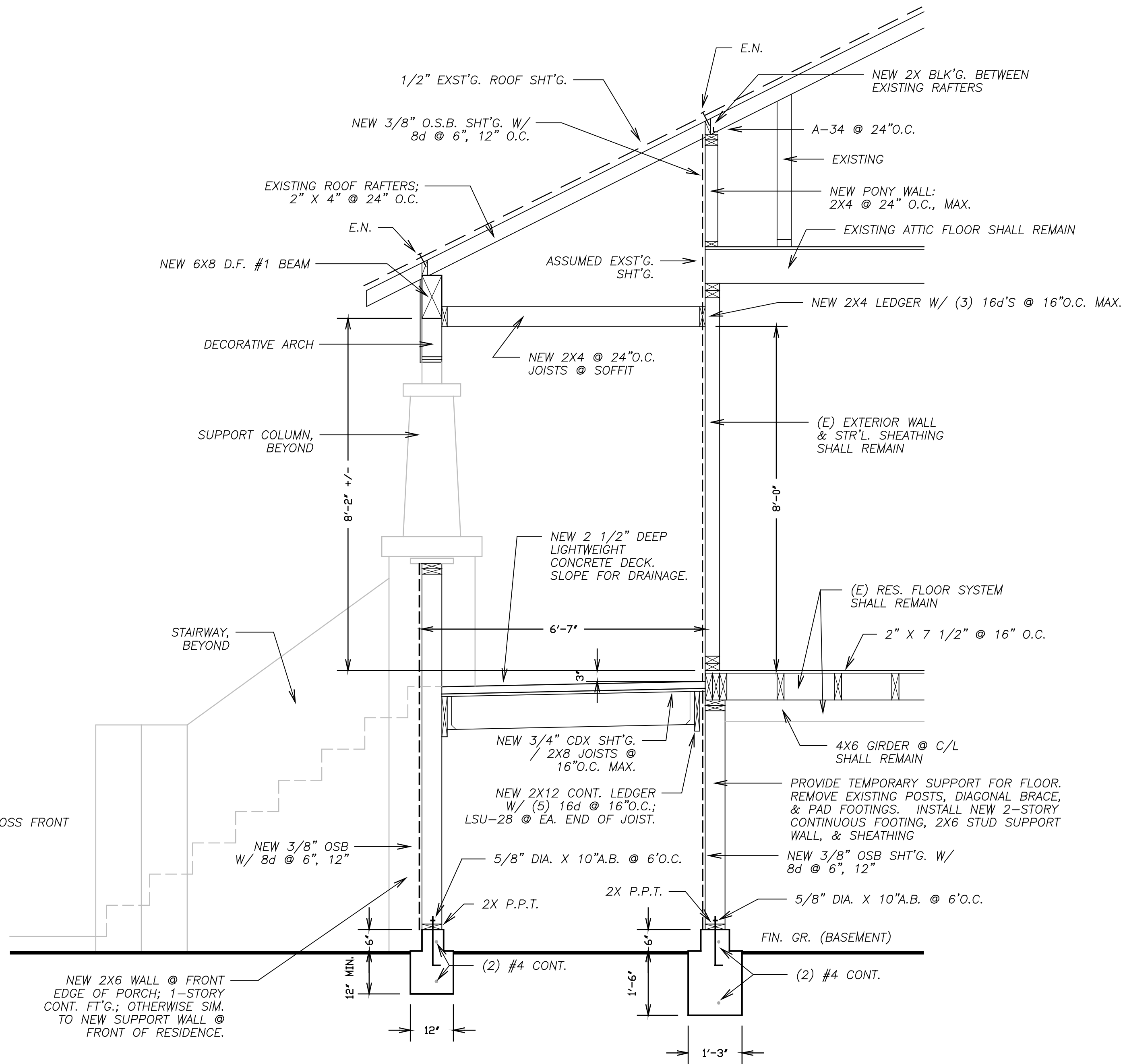
2 SEC. @ PONYWALL SCALE: 1/2" = 1'-0"
