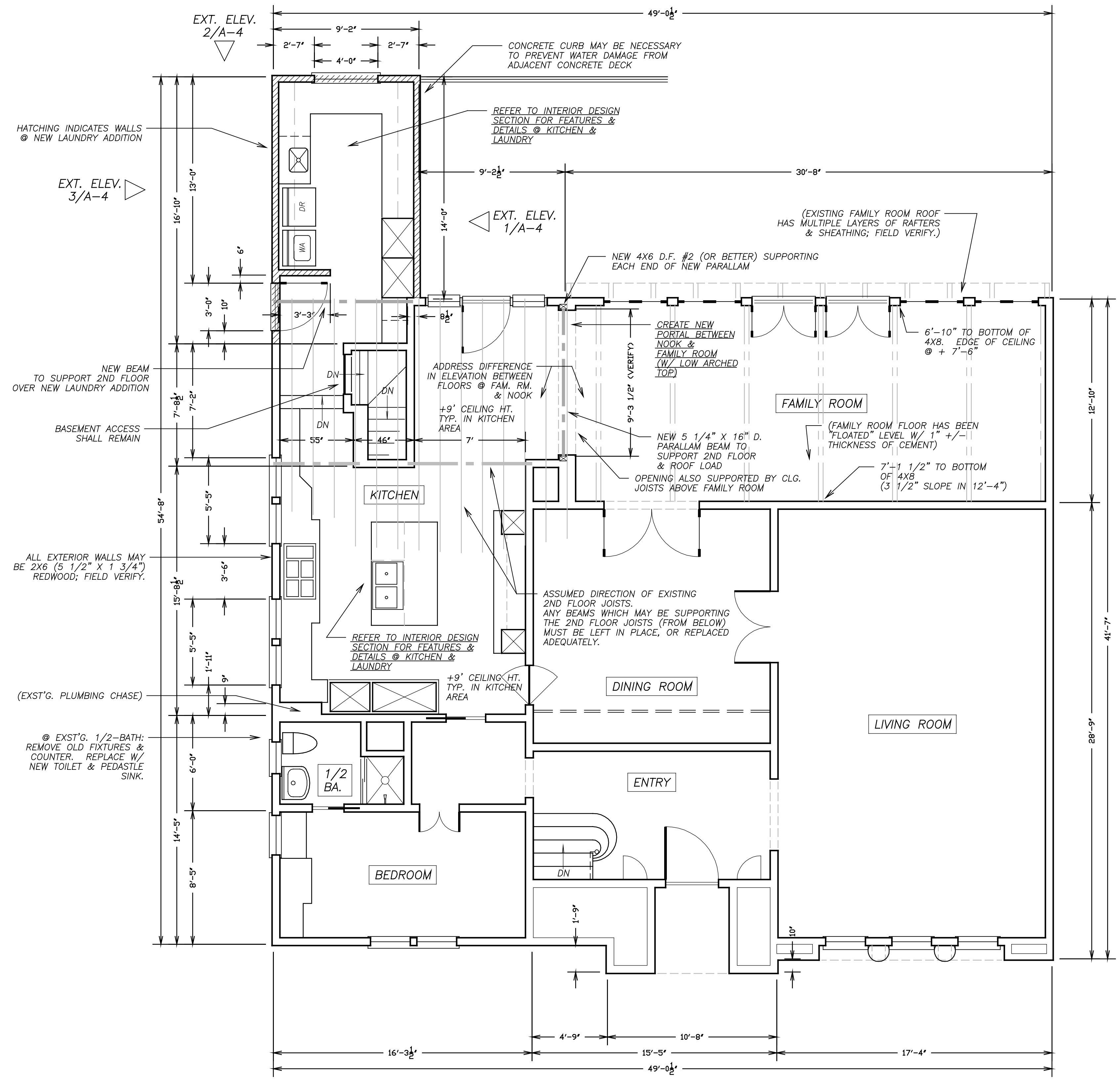
1 ADDITION & REMODEL ARCH'L. PLAN @ FIRST FLOOR SCALE: 1/4" = 1'-0"
