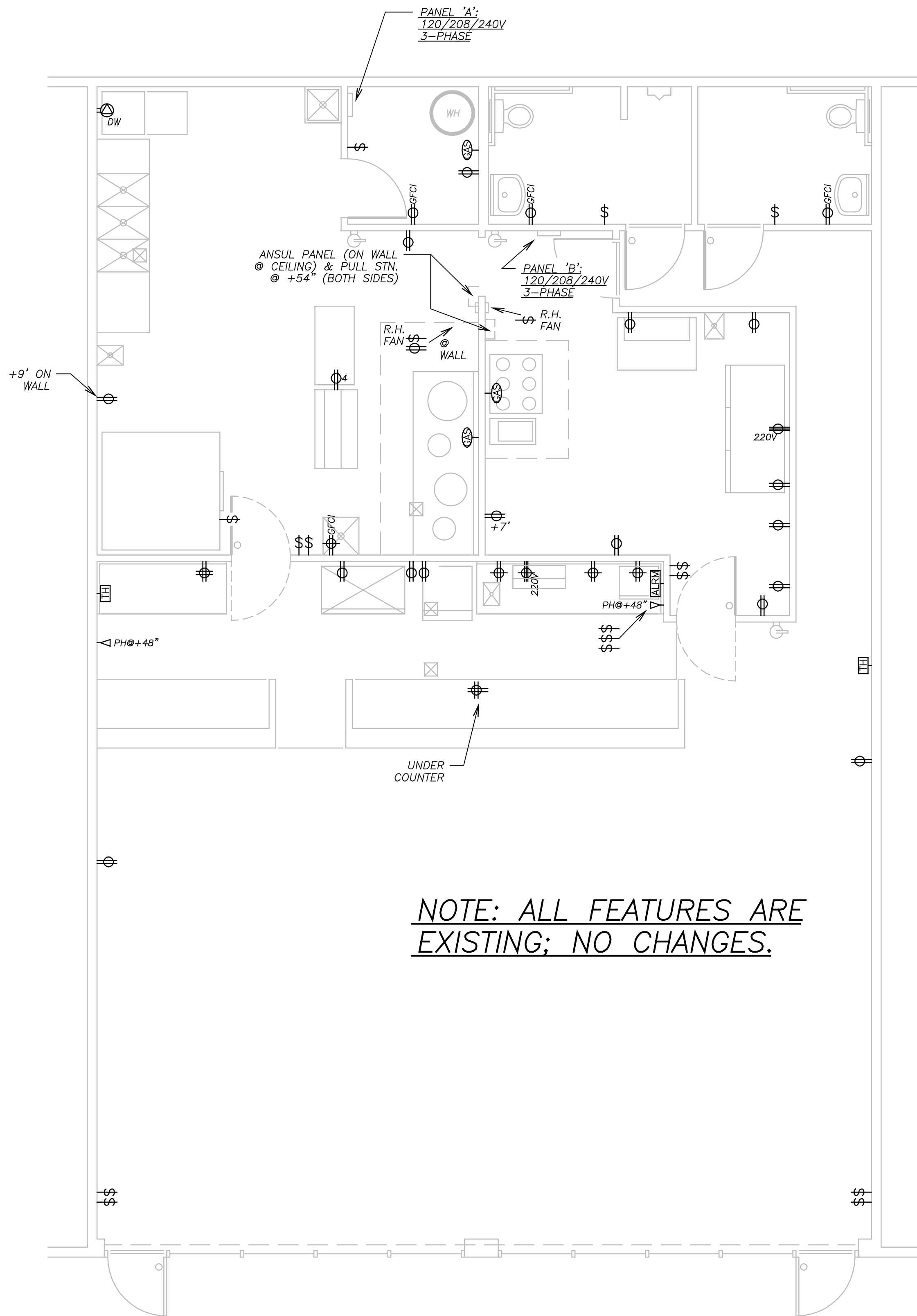
(EXISTING &) REMODEL ELECTRICAL PLAN
