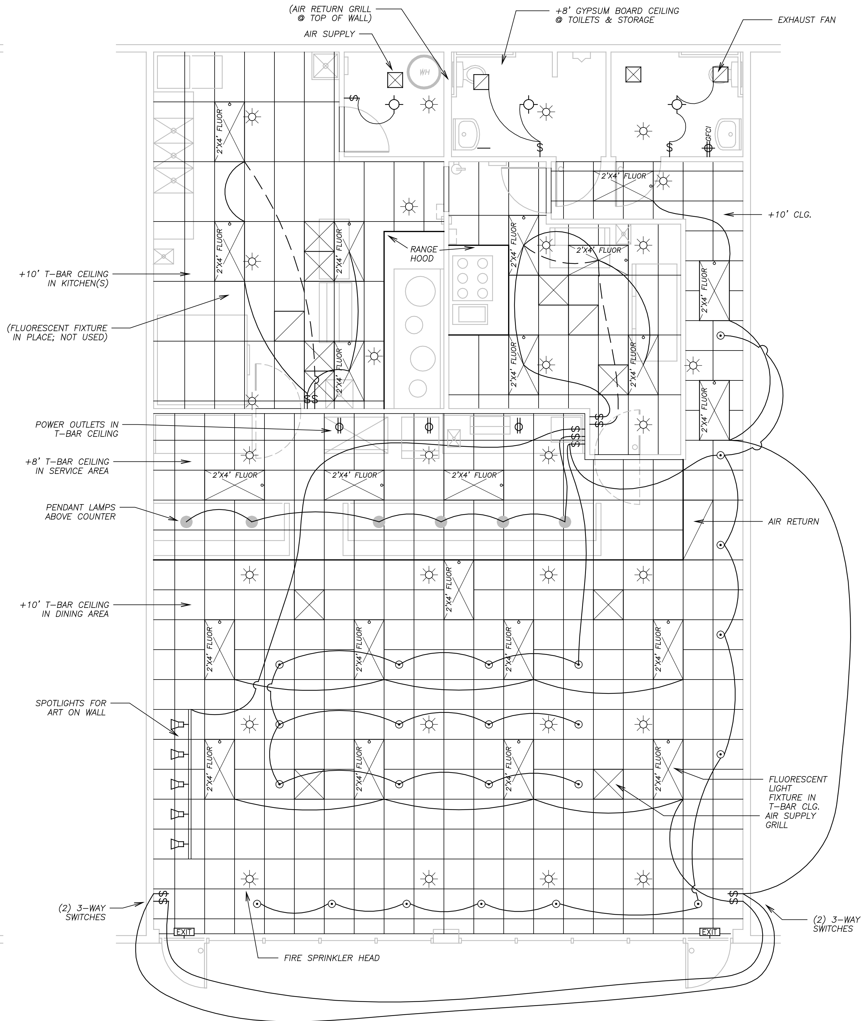
(EXISTING &) REMODEL LIGHTING PLAN
