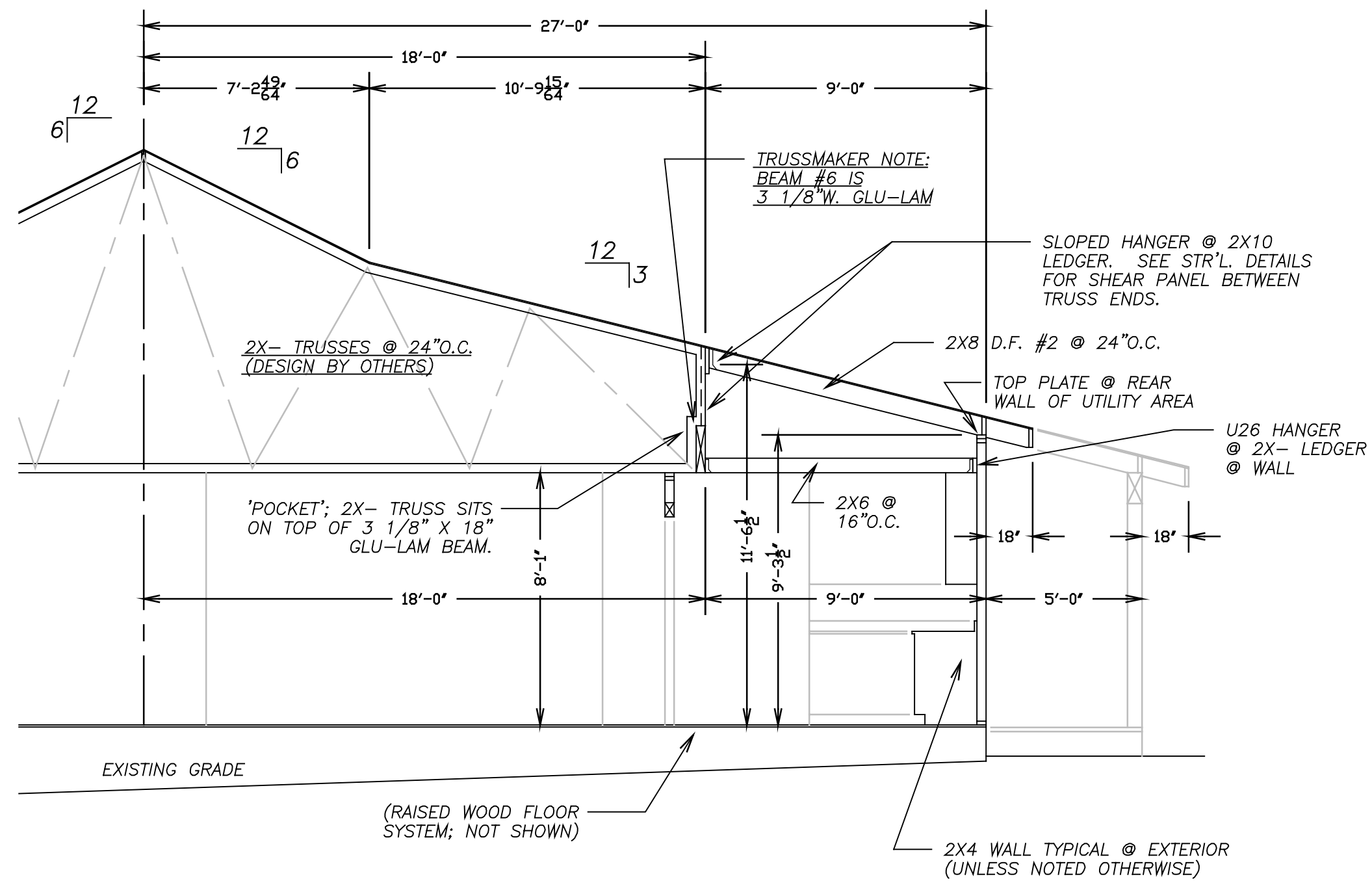
4 STRUCTURAL SECTION: #4 @ UTILITY AREA SCALE: 1/4" = 1'-0"
