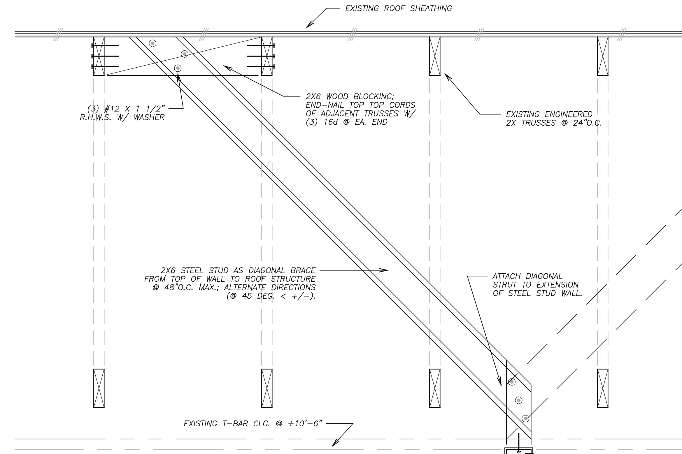
A PART'N. WALL ROOF STRUCT. SCALE: 1 1/2" = 1'-0"
