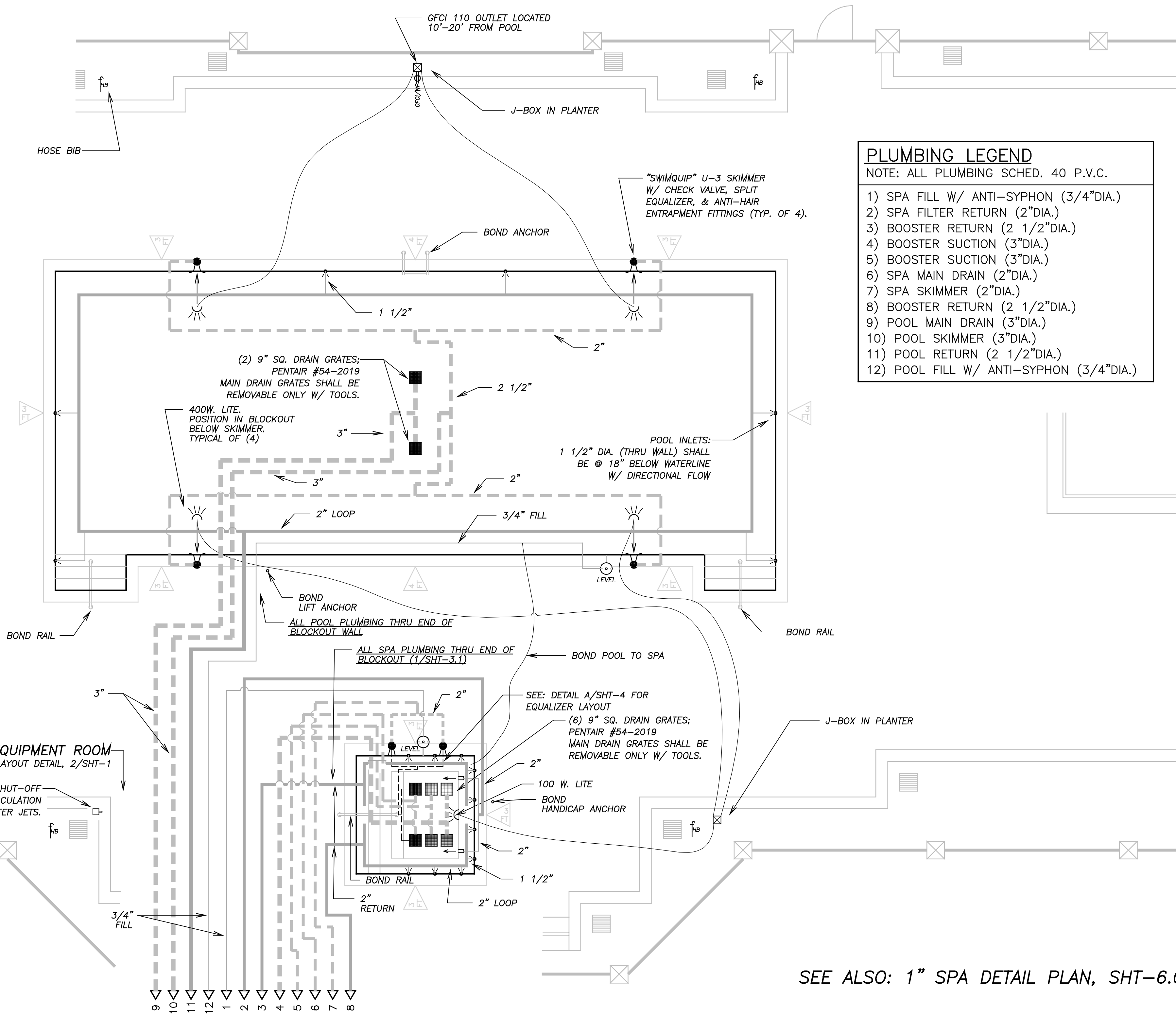
1 SITE PLUMBING PLAN SCALE: 1/4" = 1'-0"
