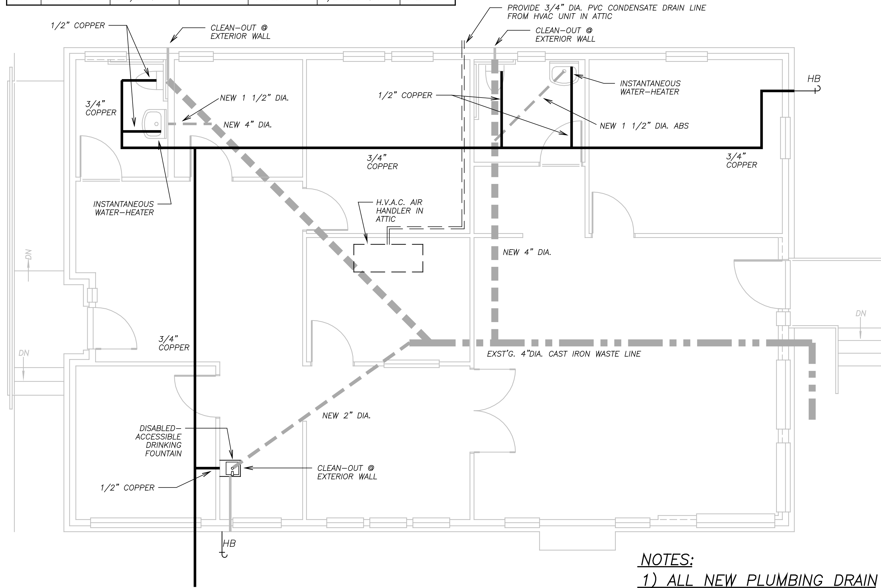
① PLUMBING SCHEMATIC FLOOR PLAN SCALE: 1/4" = 1'-0"
